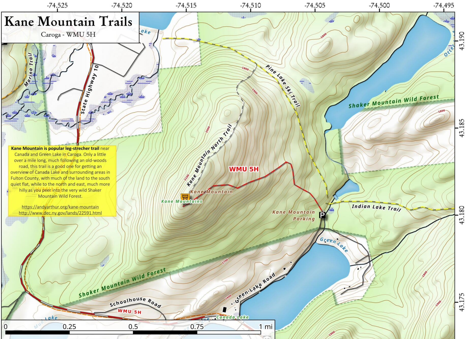
Kane Mountain Trails Map, February 24, 2019 by AndyArthur.org in QGIS 3.4.4-Madeira and Python. Street Map is Copyright © OpenStreetMap contributors, CC BY-SA. NYSDEC Data: LiDAR/DEM, Borders, ADK Wetlands, Trails, Assets. True North. 1 inch = 0.2 miles. Projection: NAD83 / UTM zone 18N. Coordinates: 0.005° latitude-longitude (WGS84). Contours are 20 feet.
