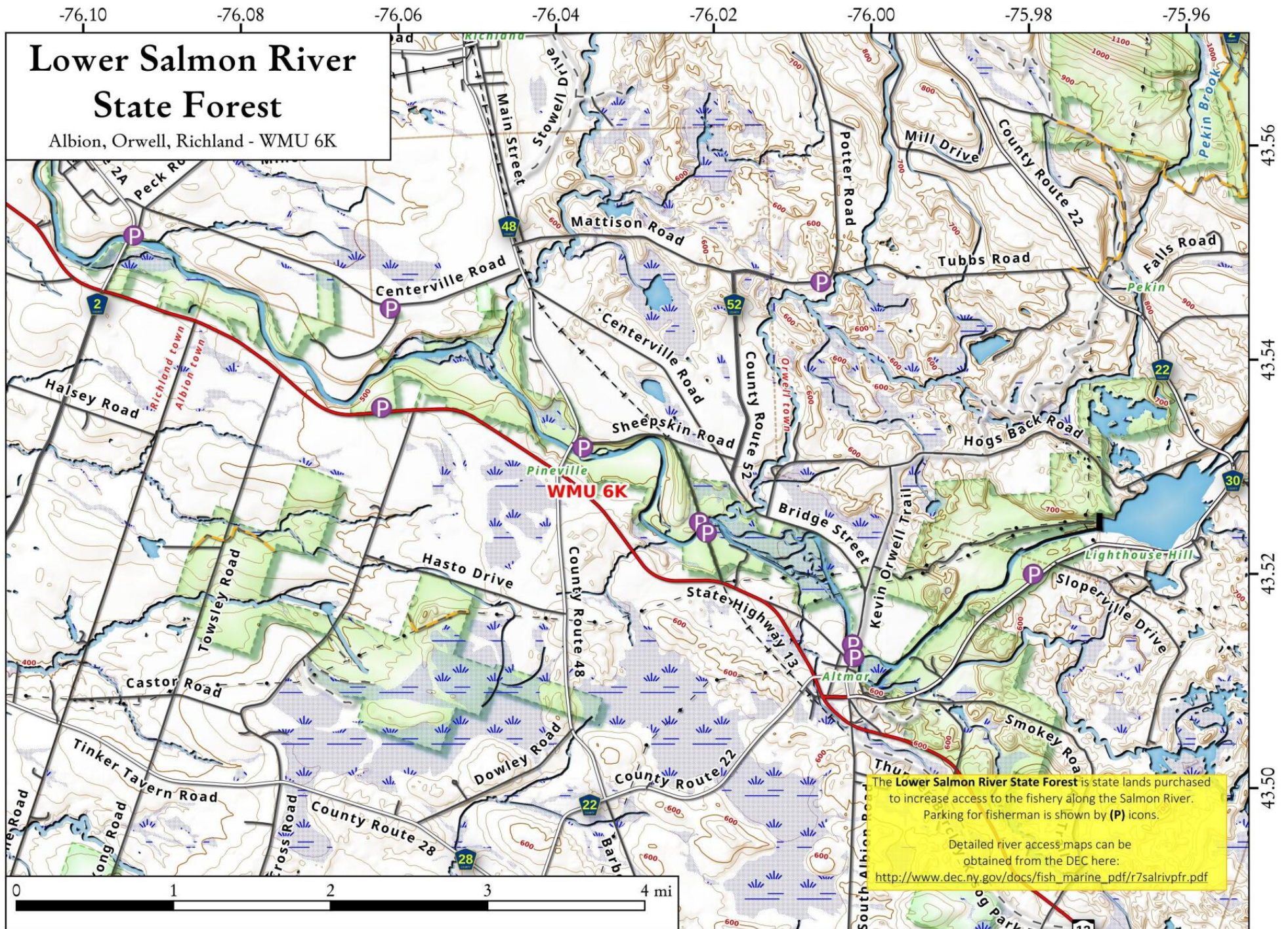
Lower Salmon River State Forest Map, November 18, 2018 by AndyArthur.org in QGIS 3.4.0-Madeira and Python. Street Map is Copyright © OpenStreetMap contributors, CC BY-SA. NYSDEC Data: LiDAR/DEM, Borders, ADK Wetlands, Trails, Assets. True North. 1 inch = 0.8 miles. Projection: NAD83 / UTM zone 18N. Coordinates: 0.02° latitude-longitude (WGS84). Contours are 20 feet.
