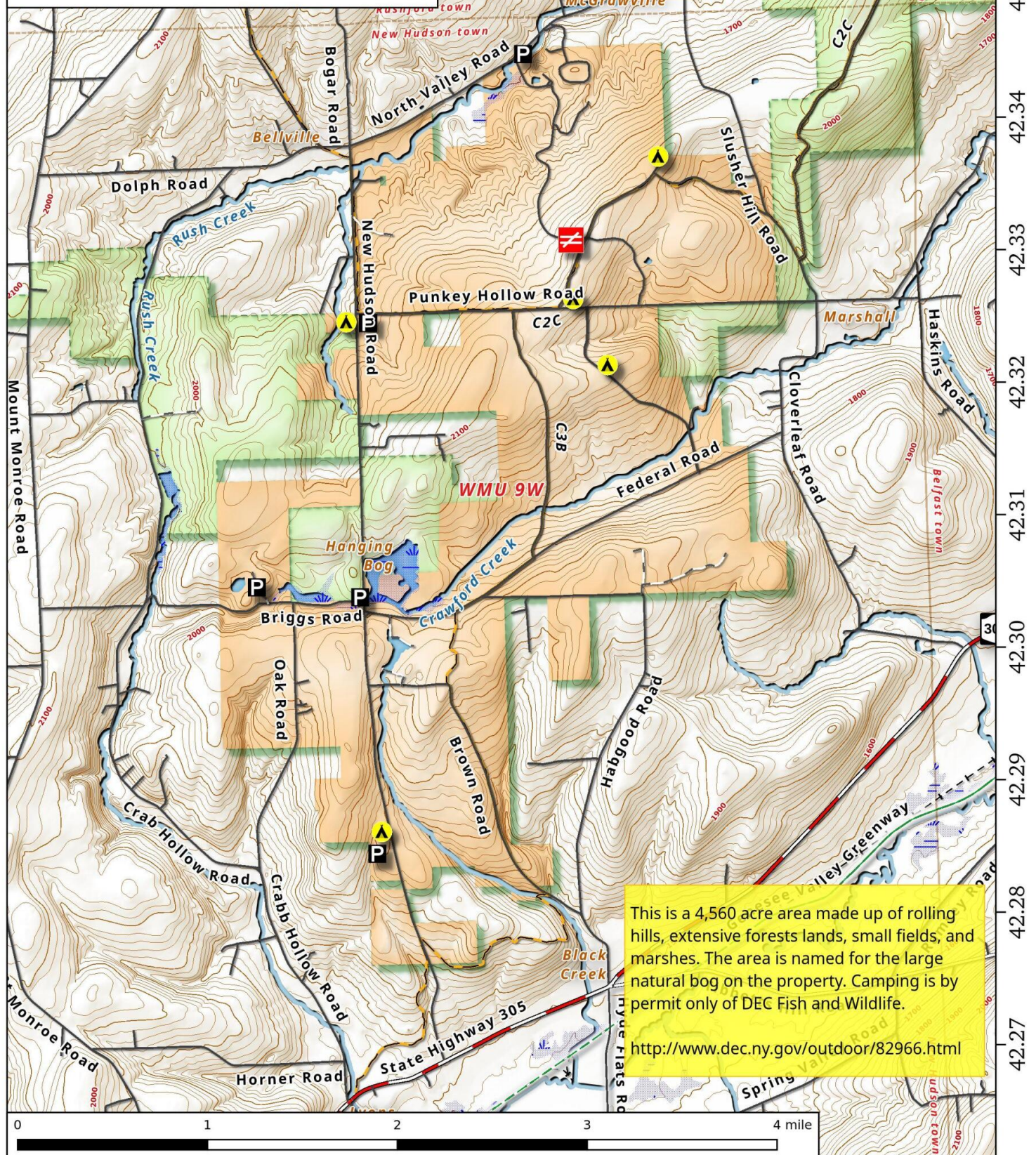
Hanging Bog Wildlife Management Area Map, March 29, 2018 by AndyArthur.org in QGIS 2.18.11 and Python. Street Map is Copyright © OpenStreetMap contributors, CC BY-SA. NYSDC Data: LiDAR/DEM, Borders, ADK Wetlands, Trails, Assets. True North. 1 inch = 0.7 miles. Projection: NAD83 / UTM zone 17N. Coordinates: 0.01° latitude-longitude (WGS84). Contours are 20 feet.
