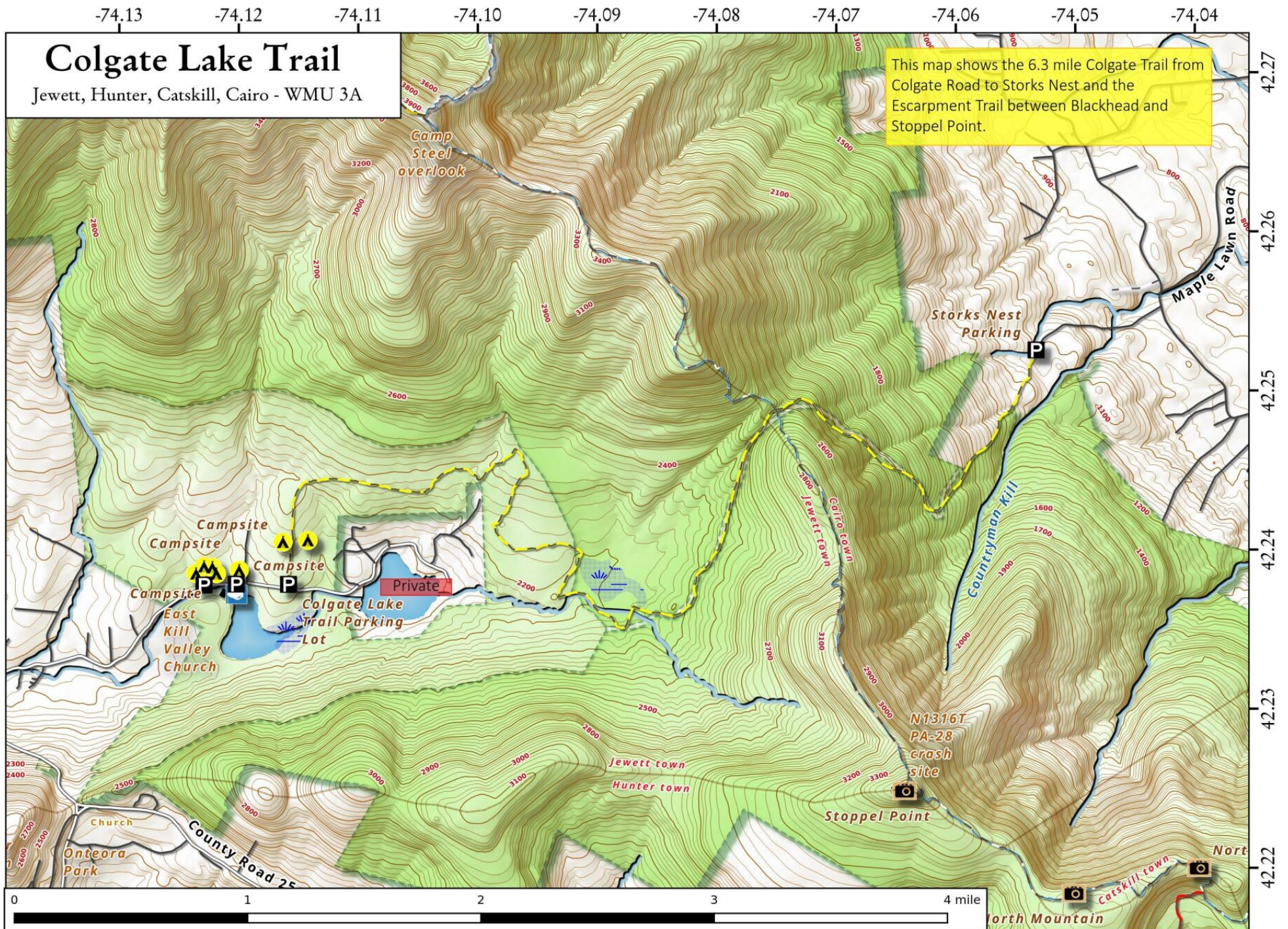
Colgate Lake Trail Map, October 9, 2017 by AndyArthur.org in QGIS 2.18.11 and Python. Street Map is Copyright © OpenStreetMap contributors, CC BY-SA. NYSDEC Data: DEM, Borders, ADK Wetlands, Trails, Assets. True North. 1 inch = 0.5 miles. Projection: NAD83 / UTM zone 18N. Coordinates: 0.01° latitude-longitude (WGS84). Contours are 20 feet.
