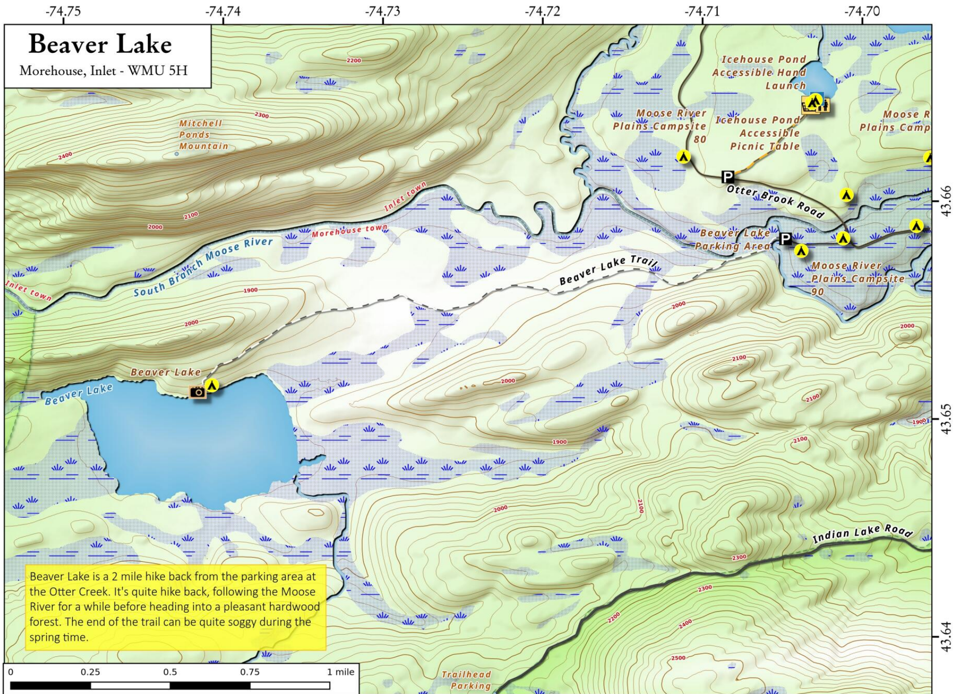
Beaver Lake Map, April 20, 2017 by AndyArthur.org in QGIS 2.18.3 and Python. Street Map is Copyright © OpenStreetMap contributors, CC BY-SA. NYSDEC Data: DEM, Borders, ADK Wetlands, Trails, Assets. True North. 1 inch = 0.3 miles. Projection: NAD83 / UTM zone 18N. Coordinates: 0.01° latitude-longitude (WGS84). Contours are 20 feet.
