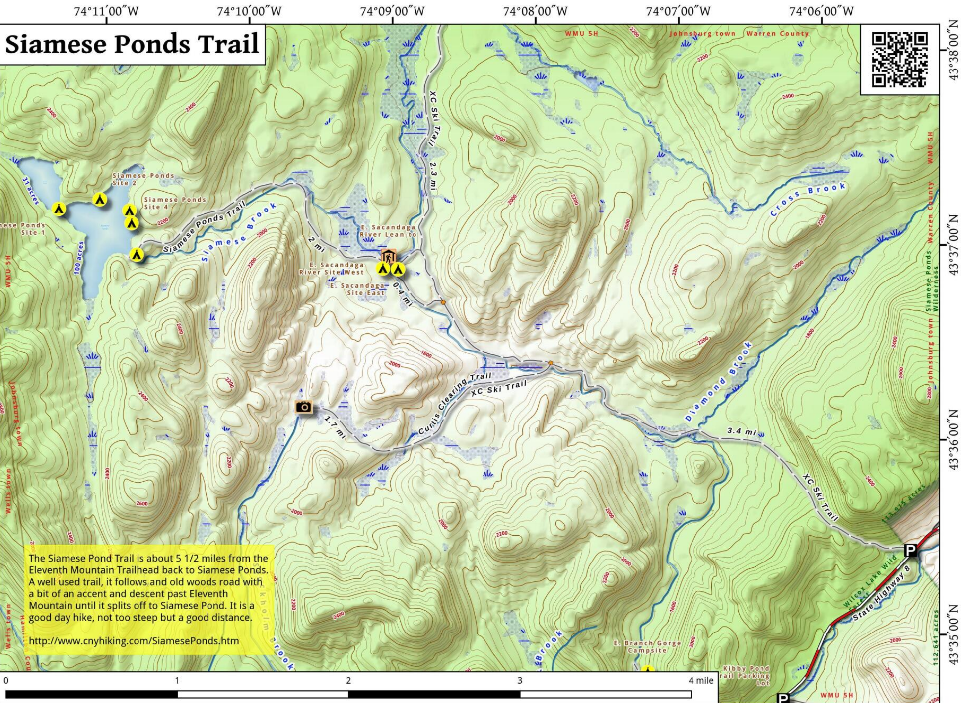
Siamese Ponds Trail Map, October 2, 2016 by AndyArthur.org in QGIS 2.16.1-Nødebo and Python. Street Map is Copyright © OpenStreetMap contributors, CC BY-SA. NYSDEC Data: DEM, Borders, ADK Wetlands, Trails, Assets. True North. 1 inch = 0.5 miles. Projection: NAD83 / UTM zone 18N. Coordinates: 60" WGS 84. Contours are 40 feet.
