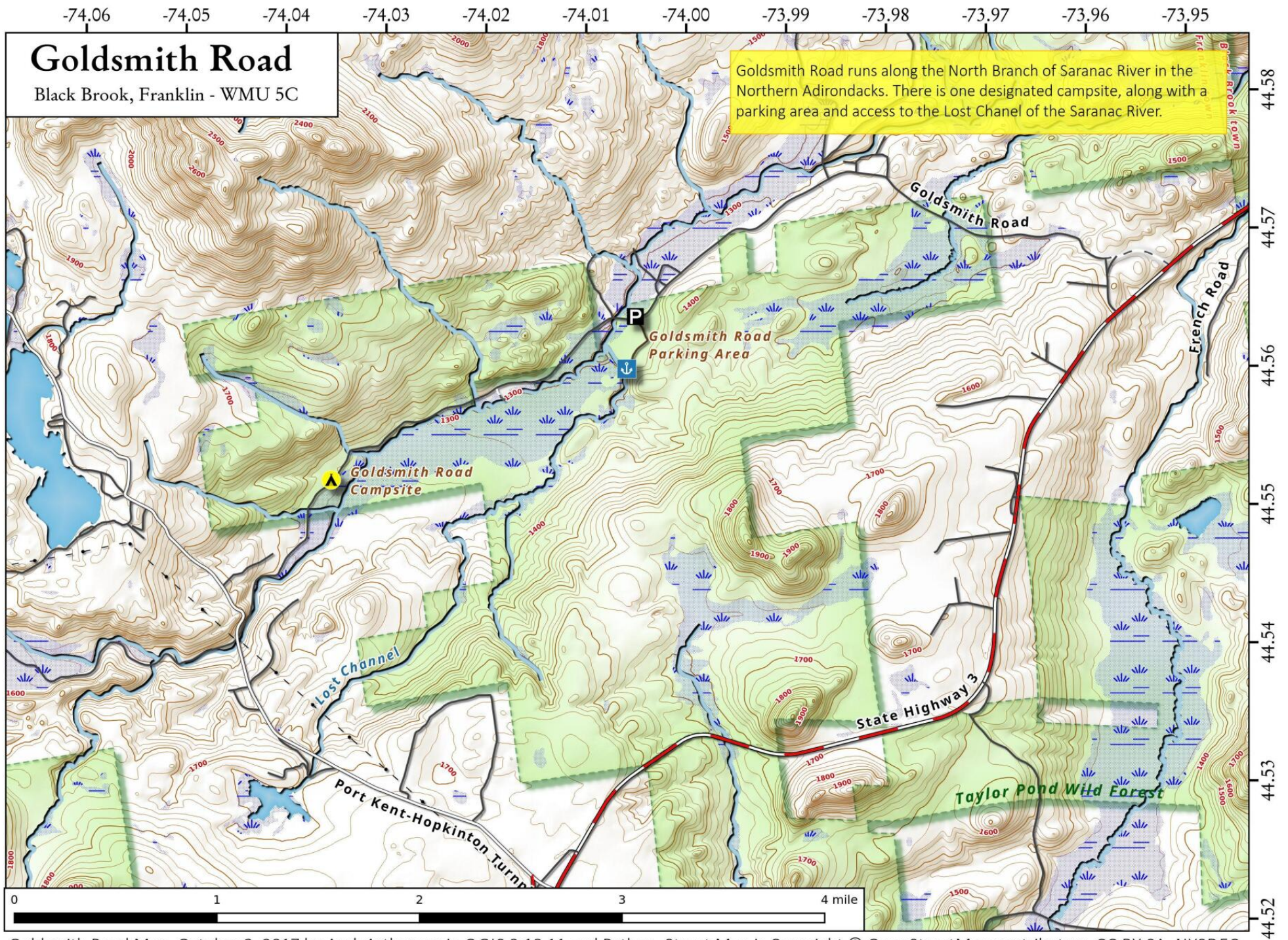
Goldsmith Road Map, October 3, 2017 by AndyArthur.org in QGIS 2.18.11 and Python. Street Map is Copyright © OpenStreetMap contributors, CC BY-SA. NYSDEC Data: DEM, Borders, ADK Wetlands, Trails, Assets. True North. 1 inch = 0.6 miles. Projection: NAD83 / UTM zone 18N. Coordinates: 0.01° latitude-longitude (WGS84). Contours are 20 feet.
